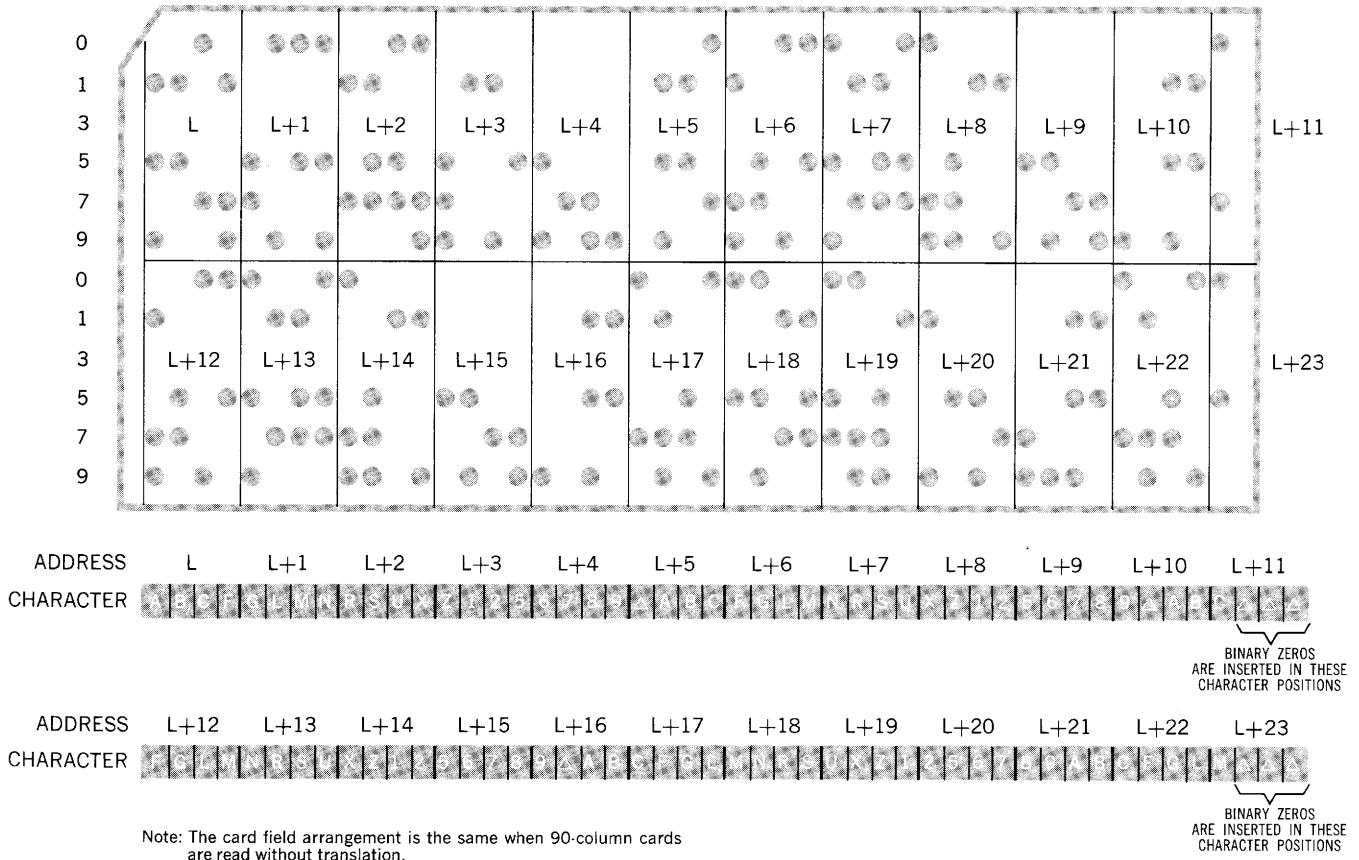
Figure 4-4. Data Transfer from Reader to Memory, With Translation, 90-Column Card
