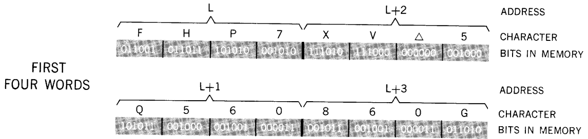
Figure 4-3. Data Transfer from Reader to Memory, Without Translation, 80-Column Card
