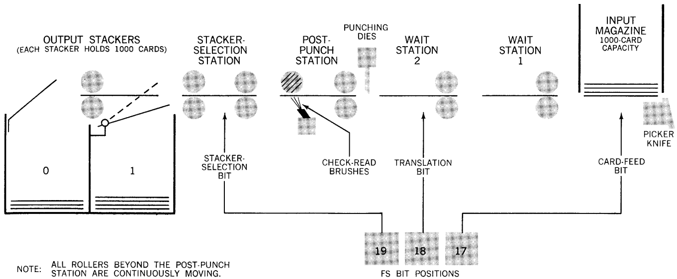
Figure 5-1. Card-Feed Path, Card-Punch Unit
