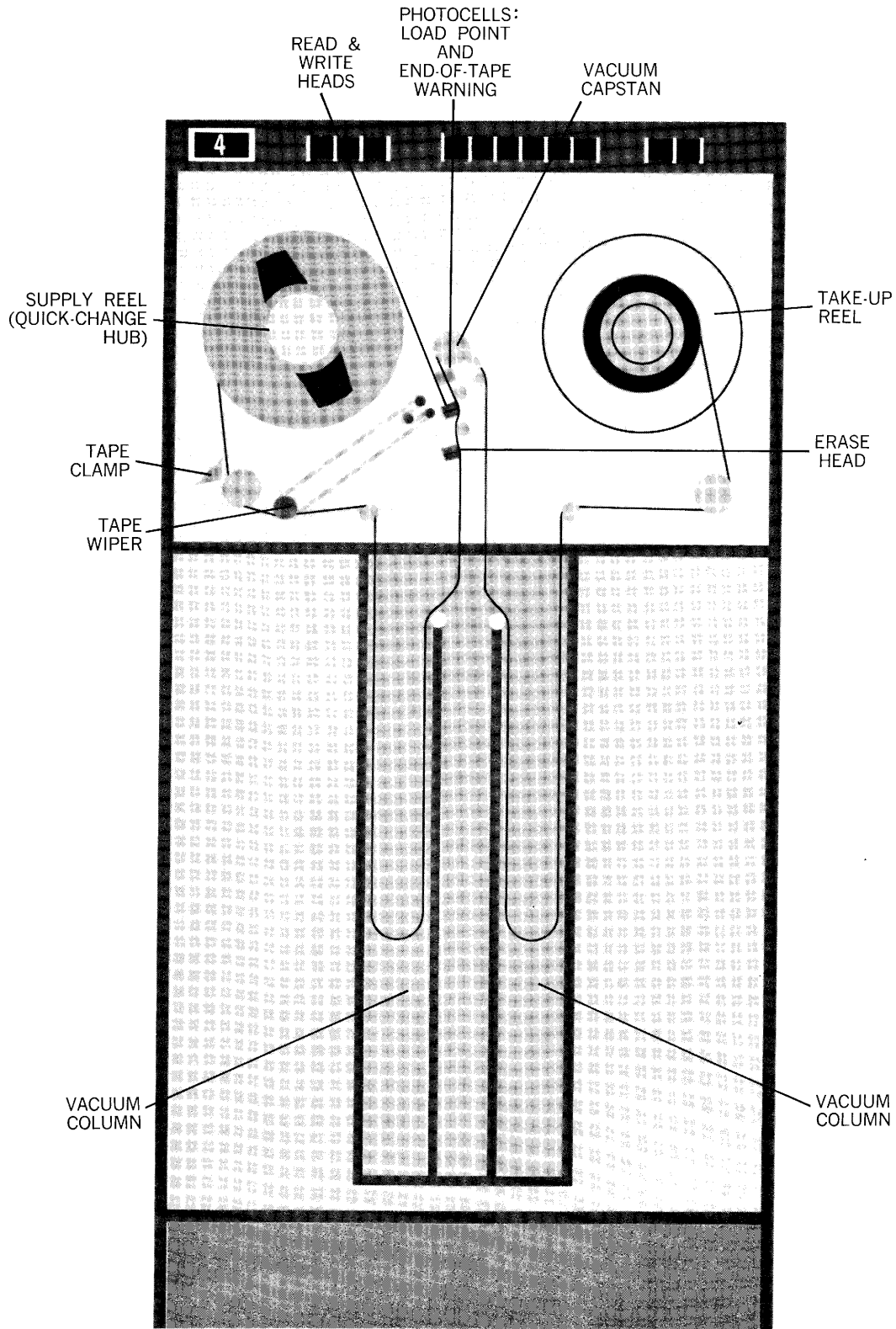
Figure 3-2. Tape Path
