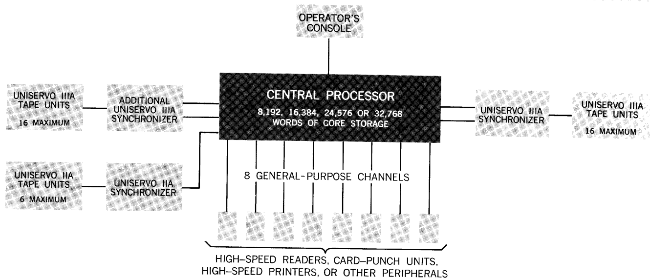
Figure 1-1. UNIVAC III System, Block Diagram
