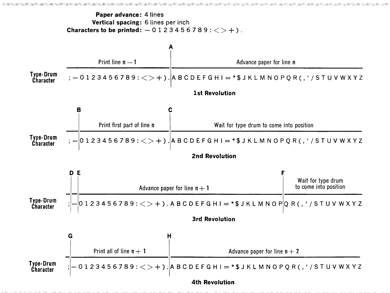
Figure F-1. Continuous Printing of Partial Character Set, Timing Diagram
