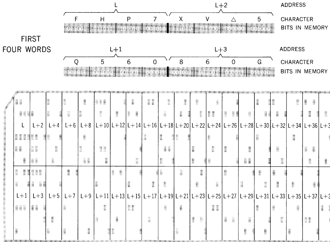
Figure 5-3. Data Transfer from Memory to Punch, Without Translation, 80-Column Card
