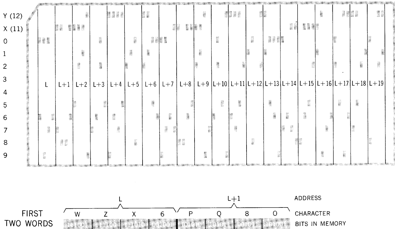
Figure 4-2. Data Transfer from Reader to Memory, With Translation, 80-Column Card
