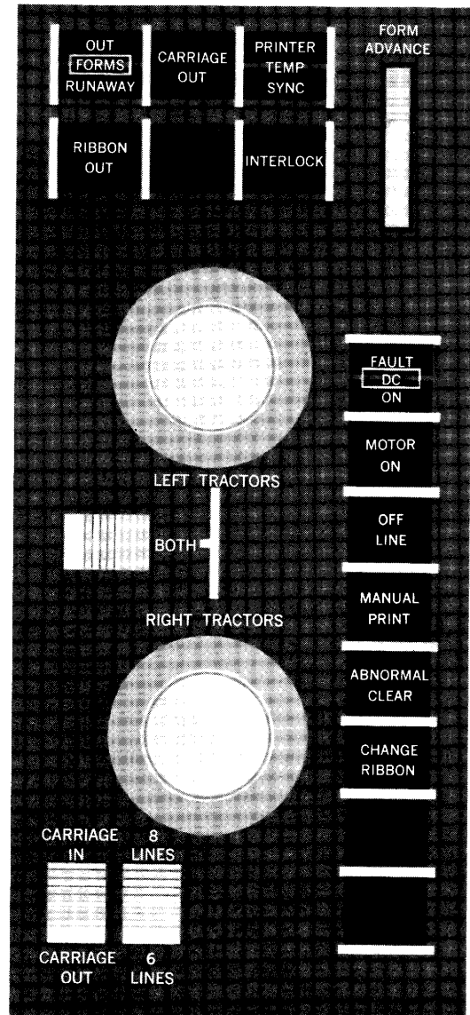
Figure 6-2. Left-Side Controls, High-Speed Printer
