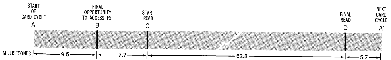
Figure 4-5. Card-Cycle Timing, High-Speed Reader
