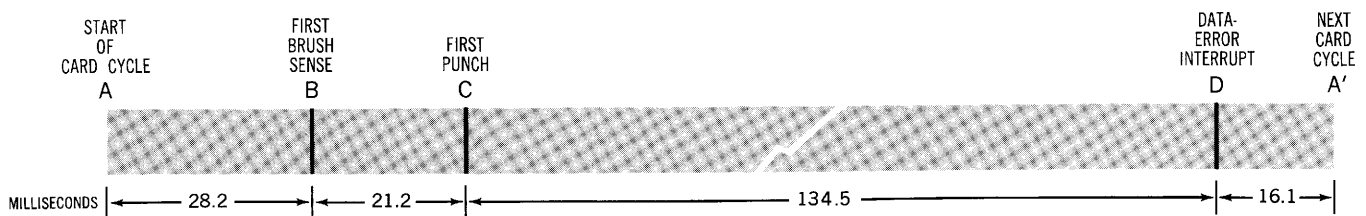
Figure 5-5. Card-Cycle Timing, Card-Punch Unit
