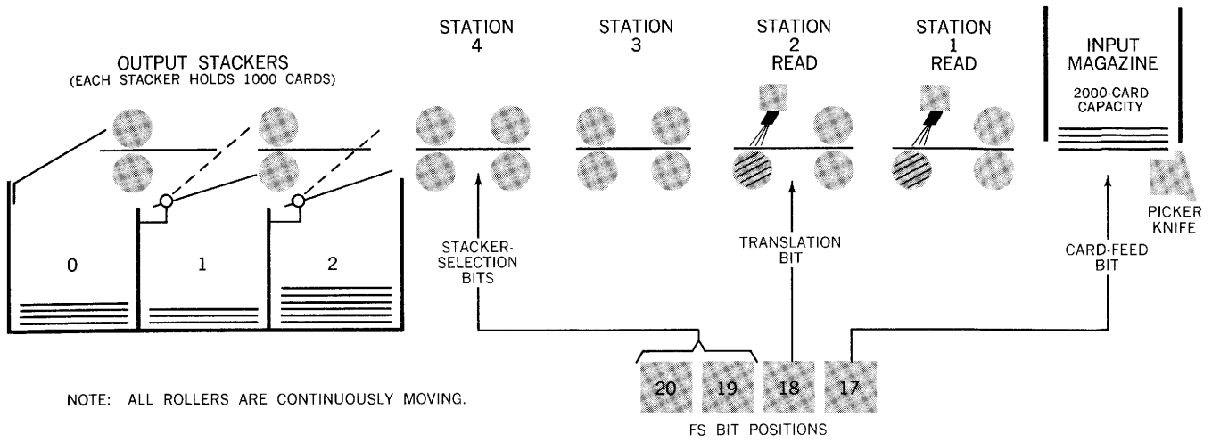
Figure 4-1. Card-Feed Path, High-Speed Reader
